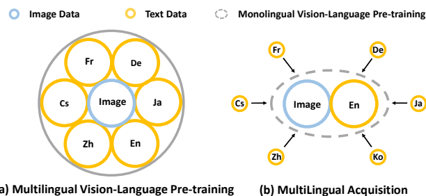
Figure 1: Comparison of data usage between M-VLP and MLA. The size of a circle reflects the amount of training data. M-VLPs learn on vision-language data from multiple languages simultaneously. Instead, MLA generalize monolingual VLP into multilingual on much less training data.
